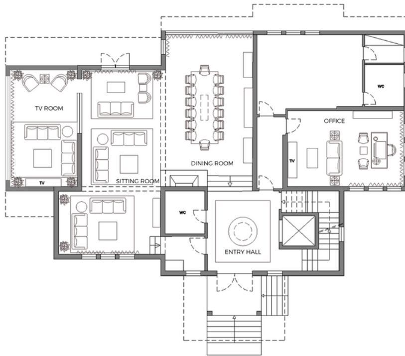
LAYOUT GROUND FLOOR
